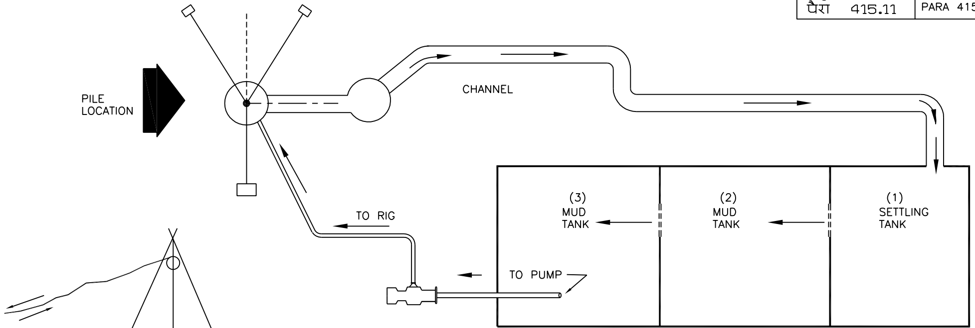
PLAN
