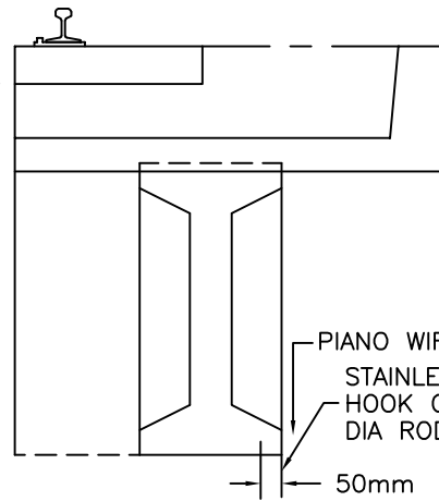
CROSS SECTION AT A-A
