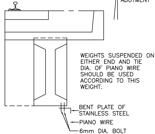
CROSS SECTION AT B-B
