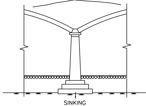
(b) CRACKS IN SPANDREL WALL DUE TO SINKING OF PIER
